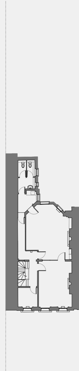
Fig.16 Existing third floor plan
