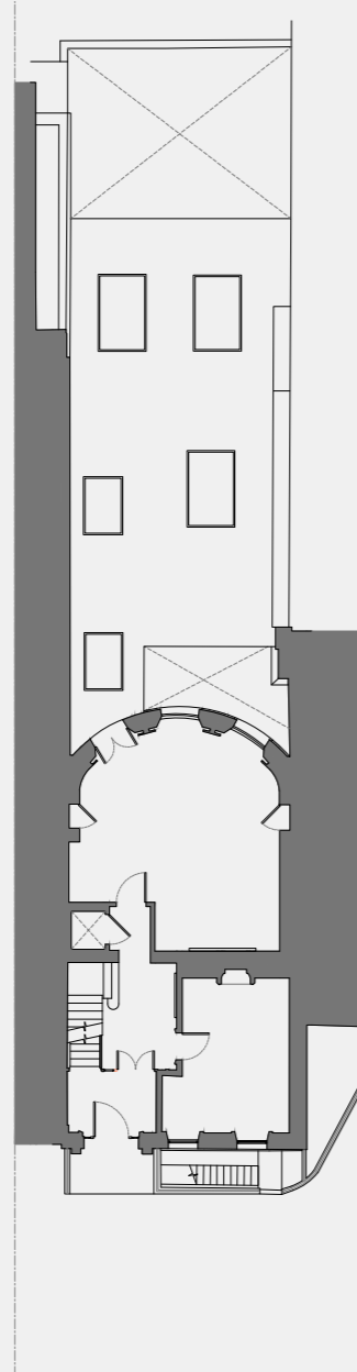
Fig.13 Existing ground floor plan
