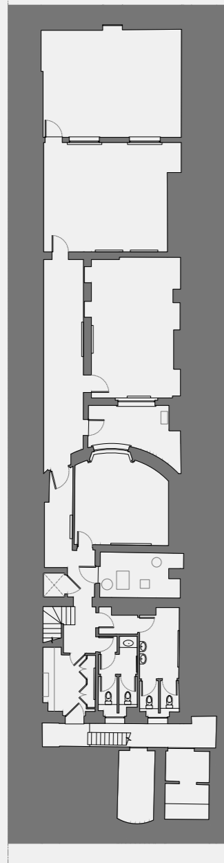
Fig.12 Existing basement plan
