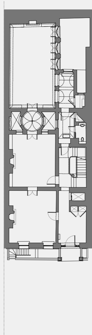
Fig.13 Existing ground floor plan
