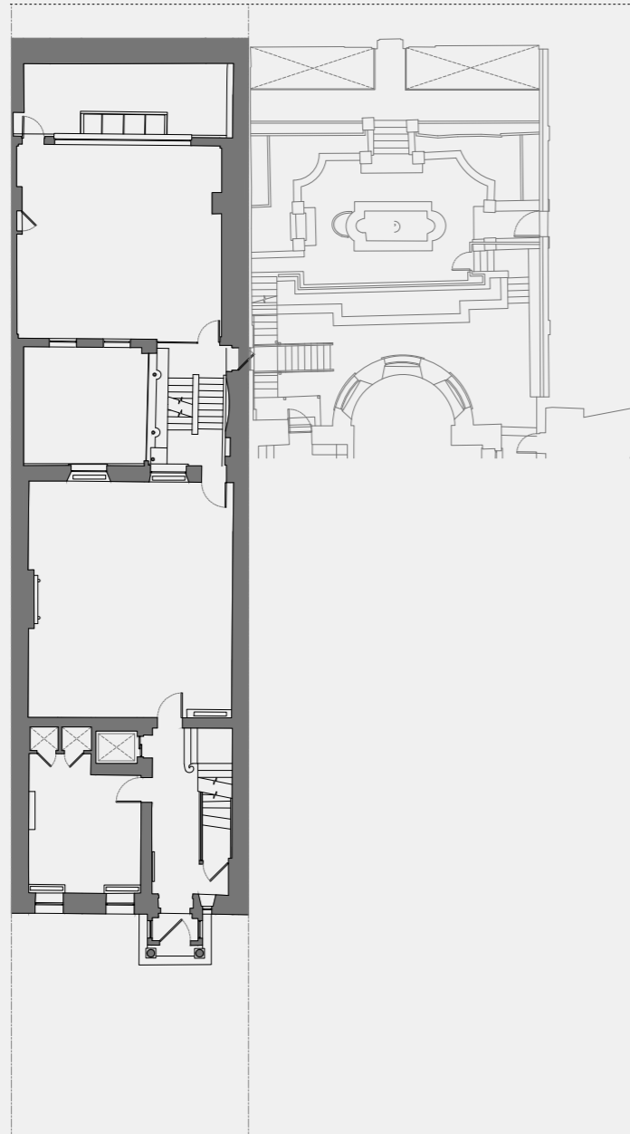
Fig.13 Existing ground floor plan
